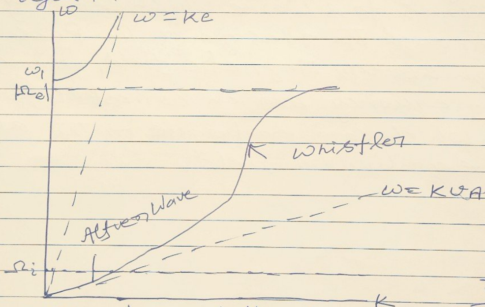
Dispersion relation for a left right handed wave propagating parallel to the magnetic field in a magnetized plasma.
